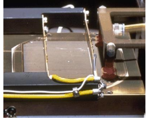
Electrical testing
